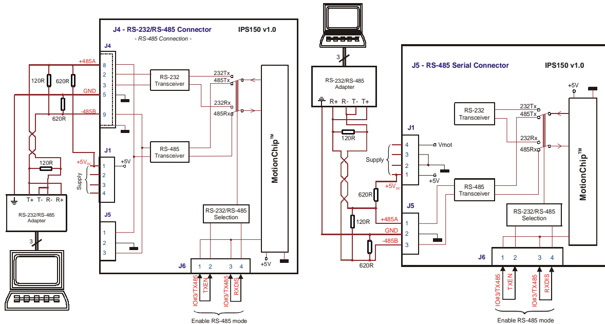
Figure 1. RS-485 connections: PC to J4 connector of IPS150. Polarity bias, applied at one network end
