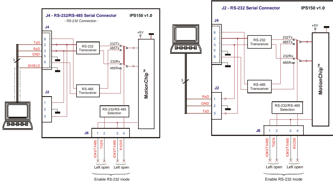
Figure A.1. RS-232 serial connections for IPS150 with J4
